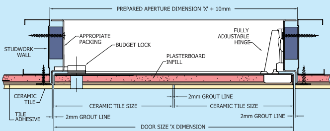
FIG 1 SECTION AA TILED WALL DOOR BUDGET LOCK OPERATED
