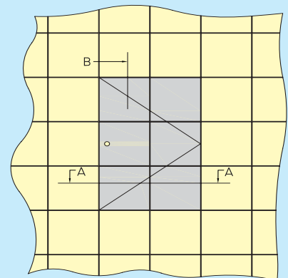
FIG 3 ELEVATION TILED WALL DOOR, BUDGET LOCK OPERATED
