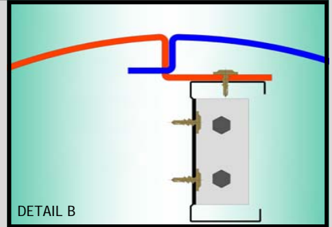
COLUMN FIXED TO INDEPENDENT STUD (FOR USE WITH STEEL SECTION COLUMN)
