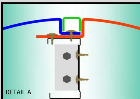
COLUMN FIXED TO INDEPENDENT STUD (FOR USE WITH STEEL SECTION COLUMN)
